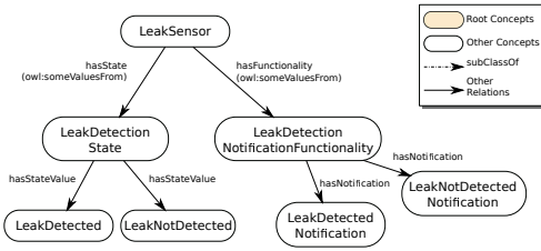
Fig. 4. An example of device class predefined in the ontology.
