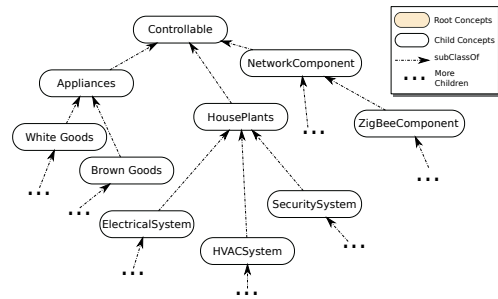
Fig. 3. Controllable subclasses.
