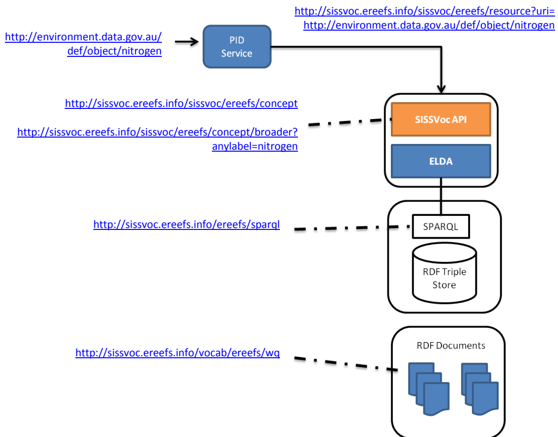
Fig. 3. A typical SISSVoc Deployment complemented by PID service and a web service hosting RDF documents. Each box represents one of the 4 different interfaces to support the various vocabulary access use cases. An additional component (labeled PID Service 9 ) redirects vocabulary URIs to the SISSVoc.
