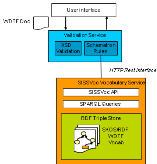
Fig. 4. WDTF Validation Service using SISSVoc Vocabulary Service
